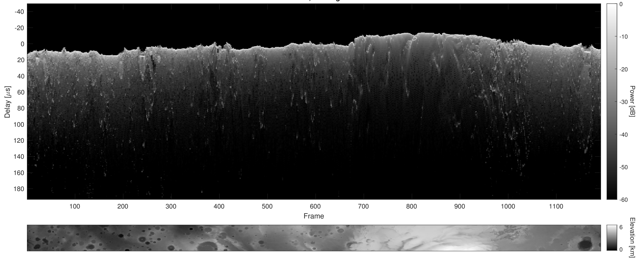
Orbit 8888, Cluttergram
