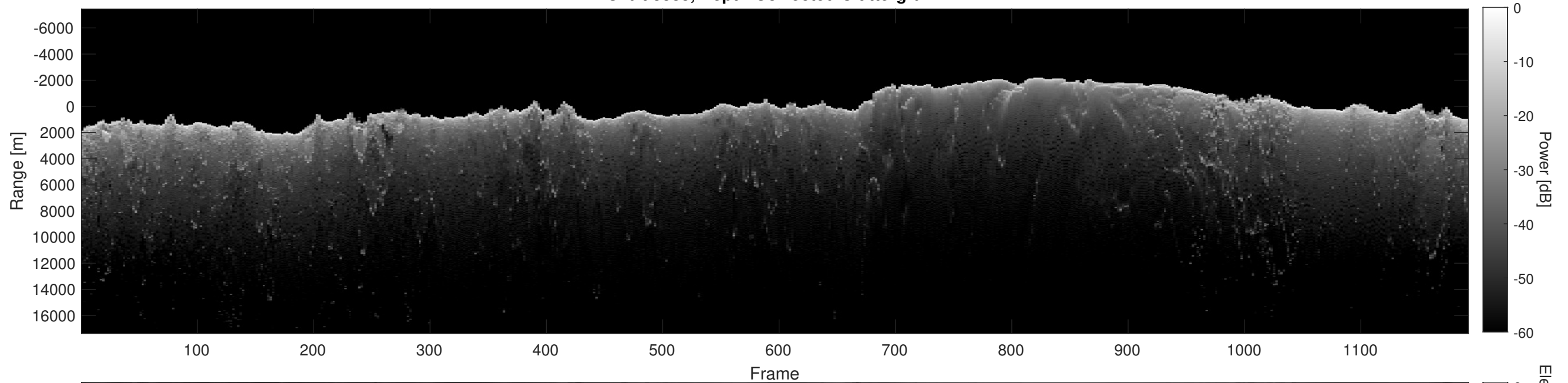
Orbit 8888, Depth-Corrected Cluttergram
