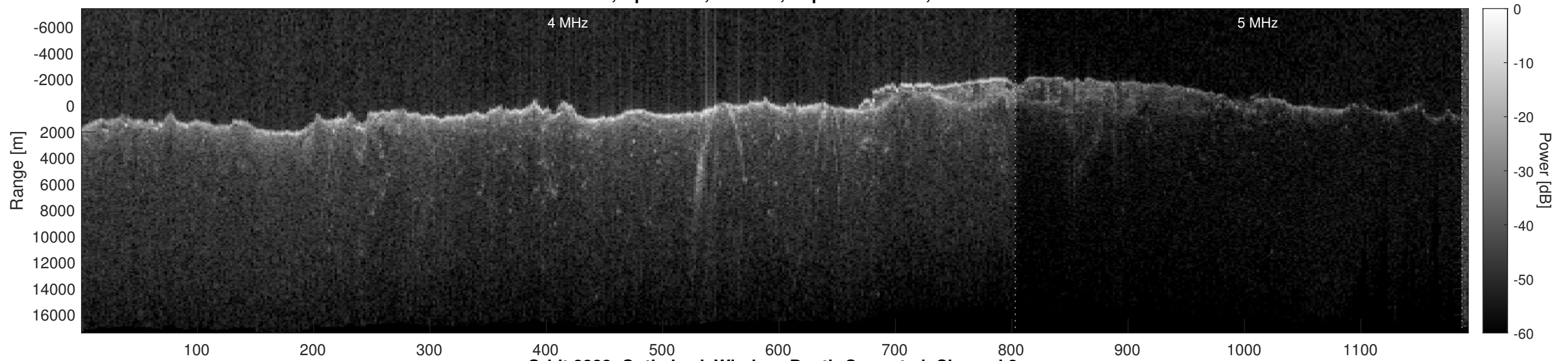
Orbit 8888, Optimized, Window, Depth-Corrected, Channel 2
