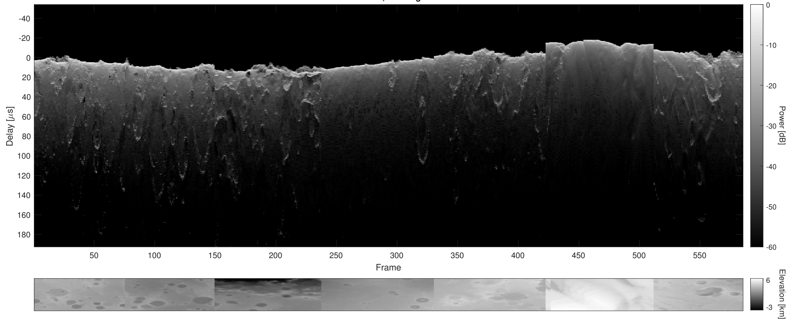
Orbit 8889, Cluttergram
