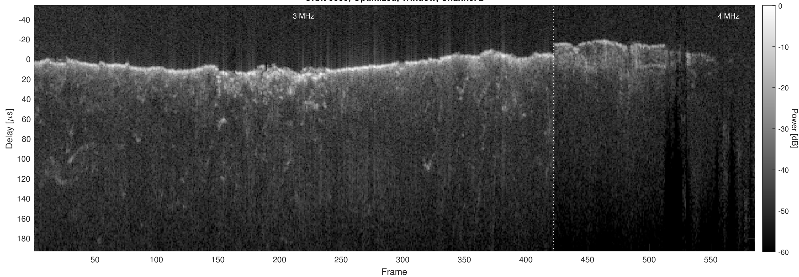
Orbit 8889, Optimized, Window, Channel 2
