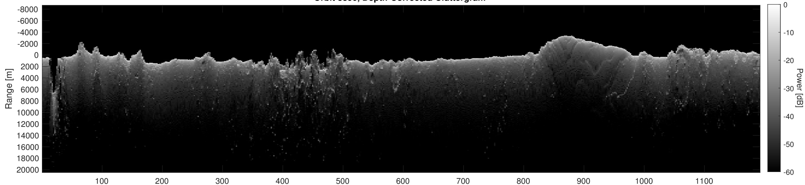
Orbit 8890, Depth-Corrected Cluttergram
