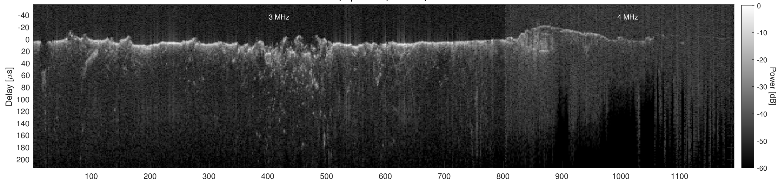
Orbit 8890, Cluttergram
