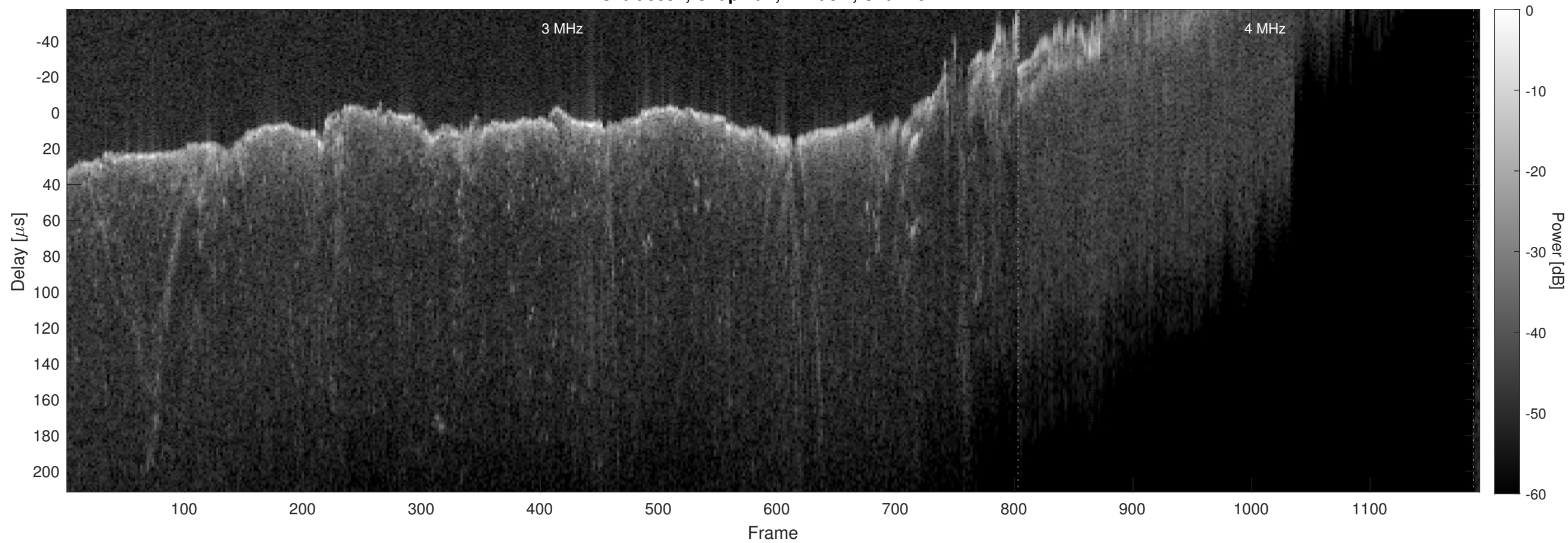
Orbit 8891, Chapman, Window, Channel 2
