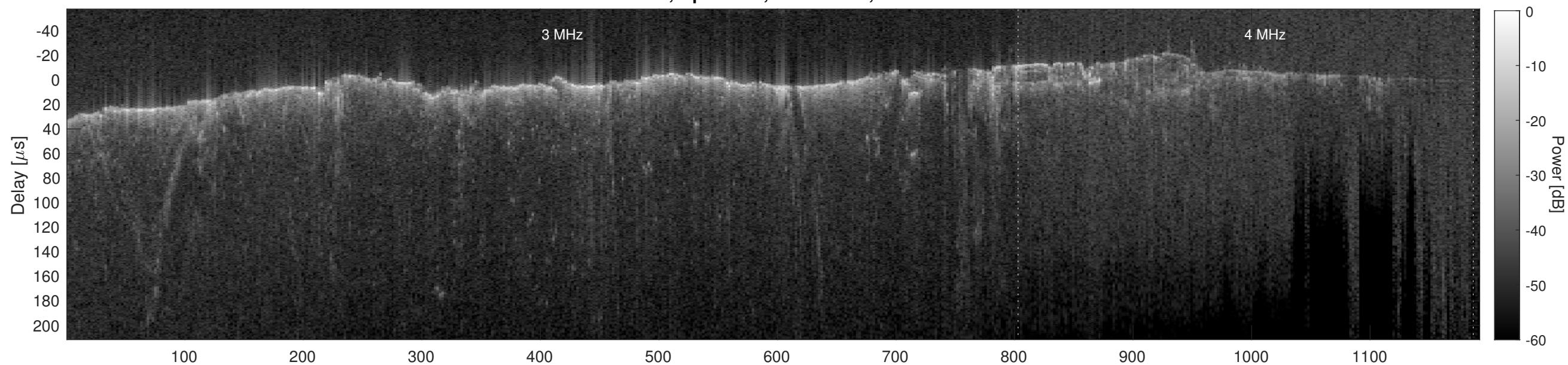
Orbit 8891, Cluttergram
