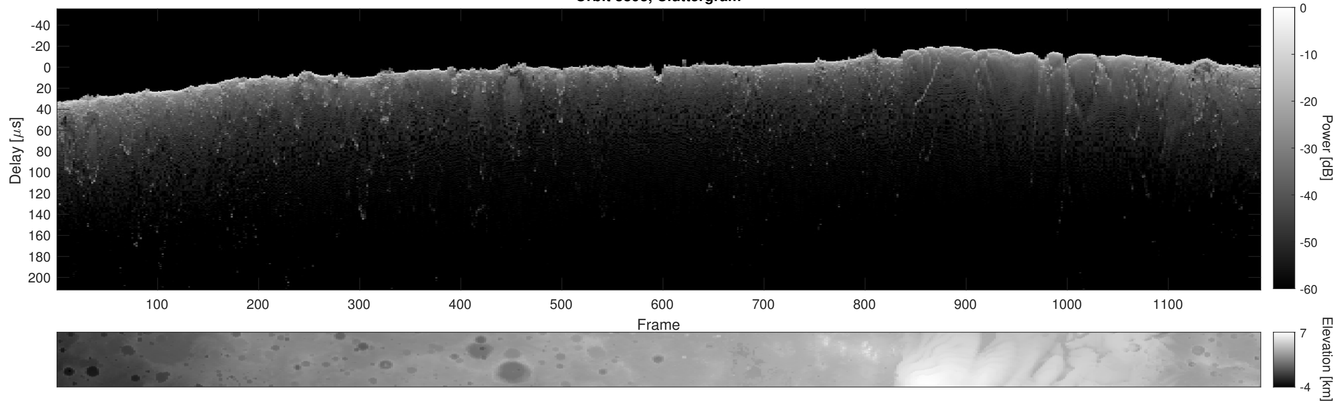
Orbit 8893, Cluttergram
