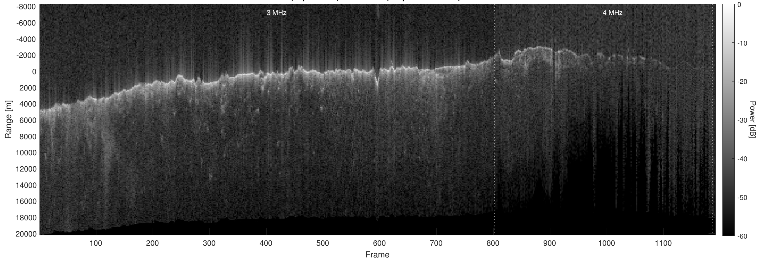
Orbit 8893, Optimized, No Window, Depth-Corrected, Channel 2
