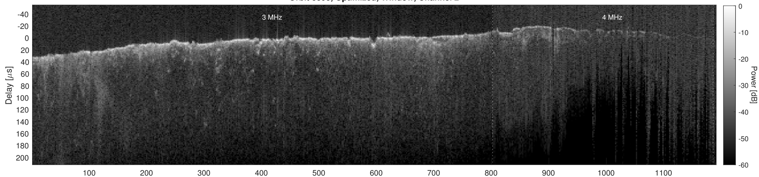
Orbit 8893, Cluttergram
