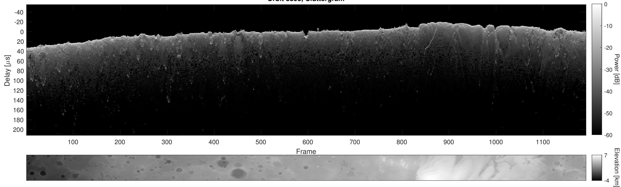
Orbit 8893, Cluttergram
