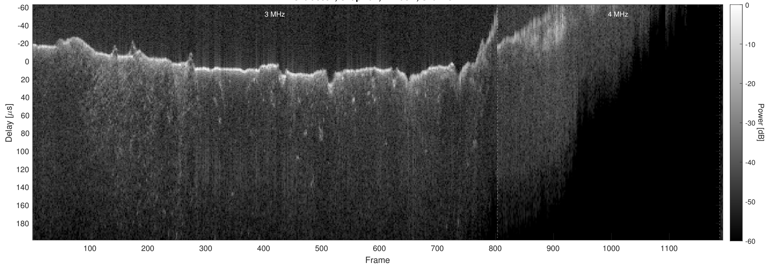
Orbit 8894, Chapman, Window, Channel 2
