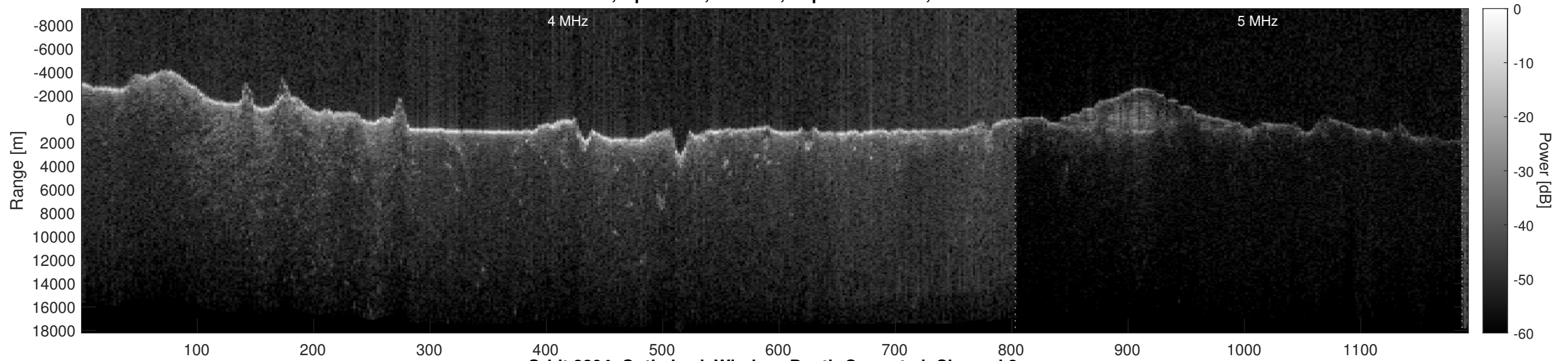
Orbit 8894, Optimized, Window, Depth-Corrected, Channel 2
