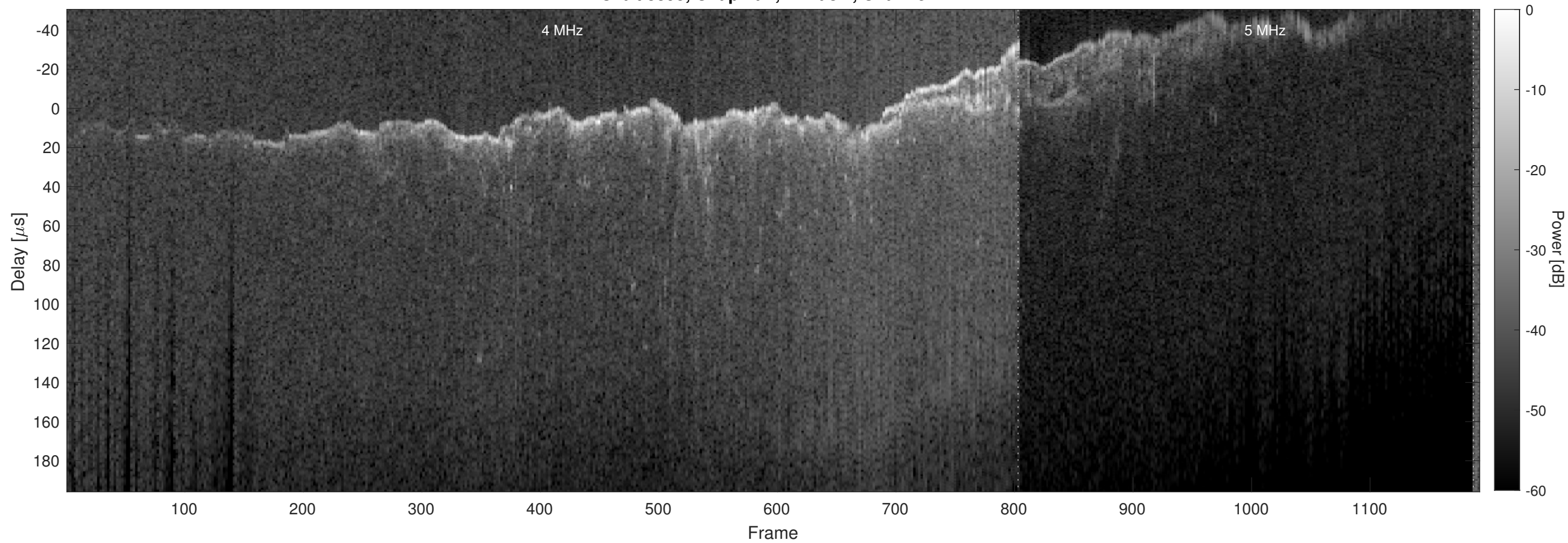
Orbit 8895, Chapman, Window, Channel 2
