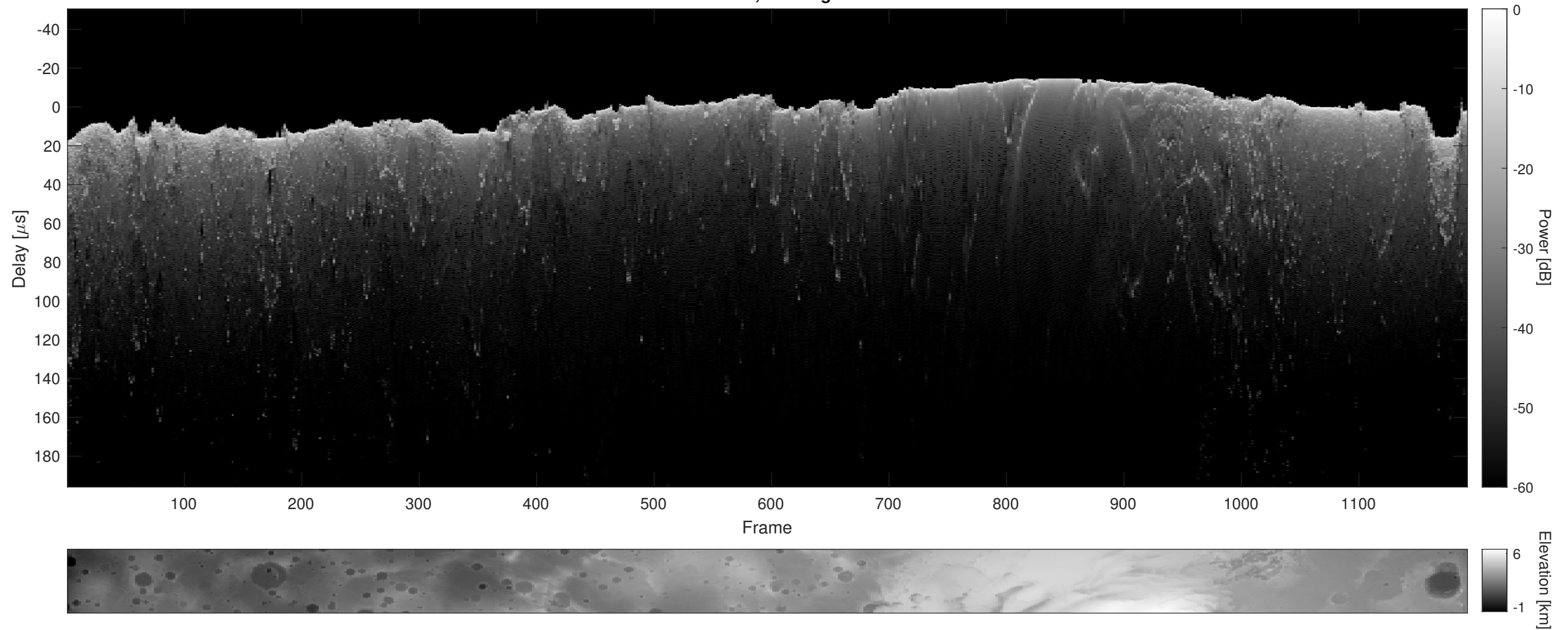
Orbit 8895, Cluttergram
