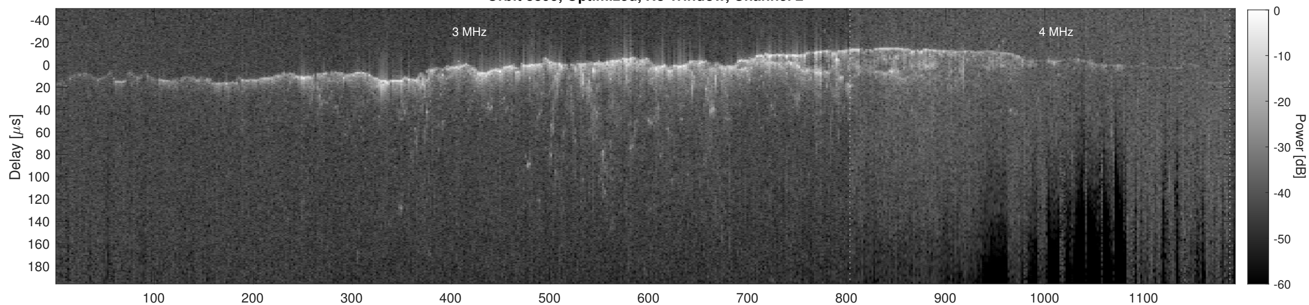
Orbit 8895, Cluttergram
