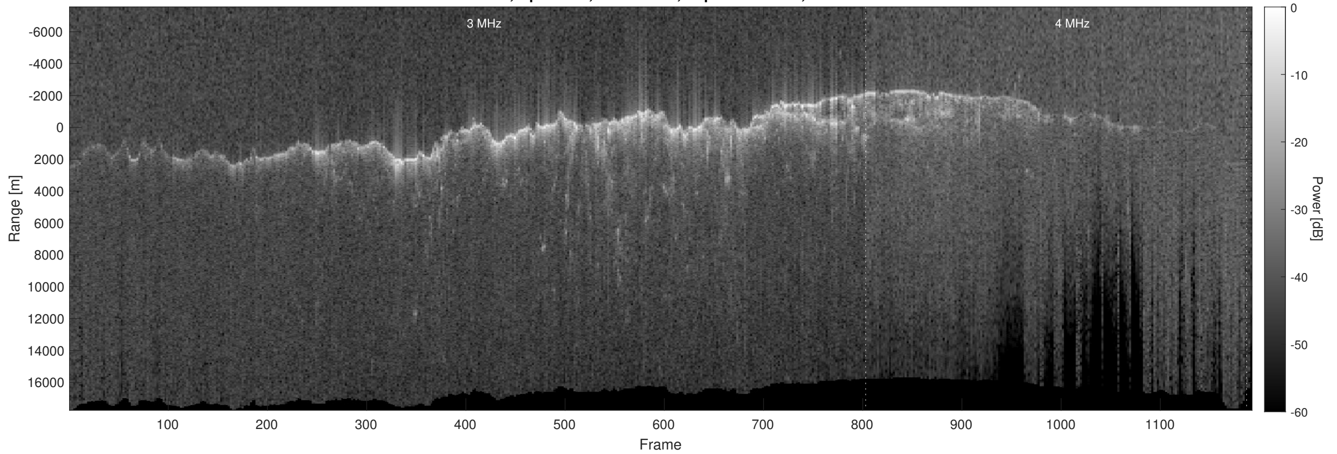
Orbit 8895, Optimized, No Window, Depth-Corrected, Channel 2
