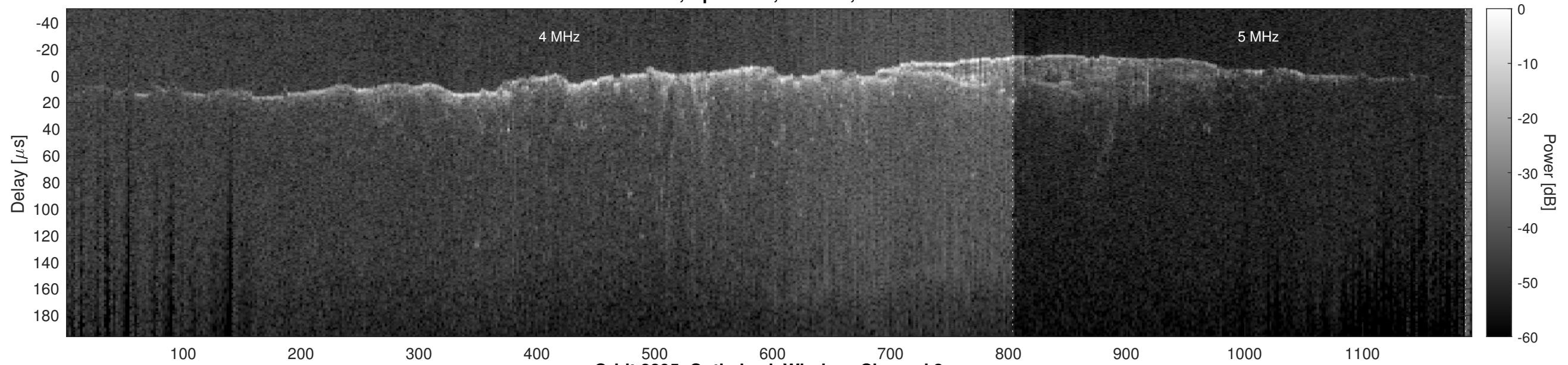
Orbit 8895, Optimized, Window, Channel 2
