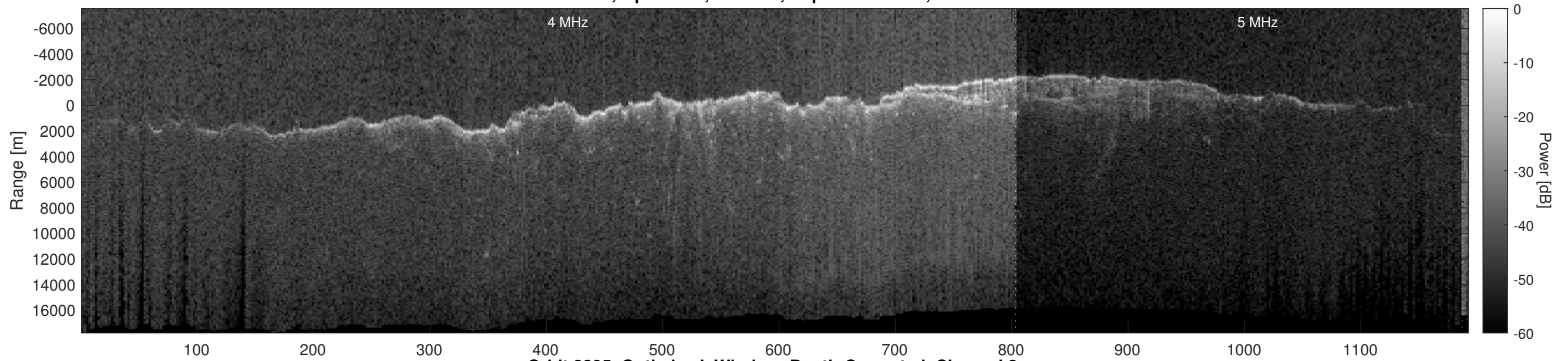
Orbit 8895, Optimized, Window, Depth-Corrected, Channel 2
