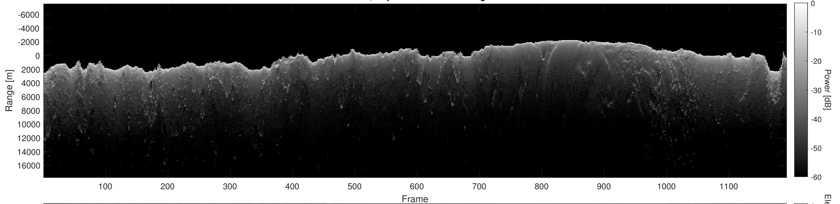
Orbit 8895, Depth-Corrected Cluttergram
