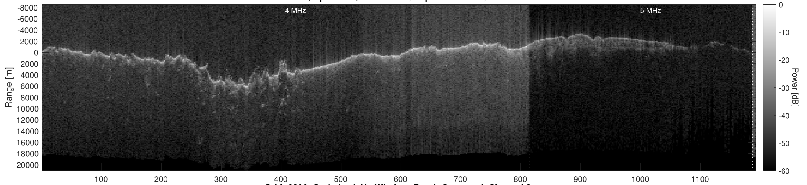
Orbit 8896, Optimized, No Window, Depth-Corrected, Channel 2
