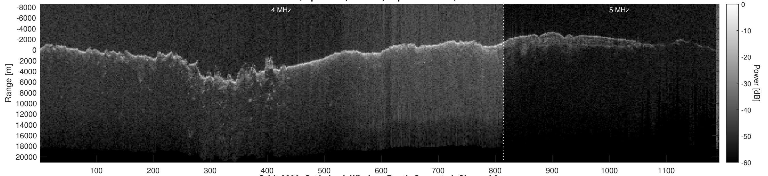
Orbit 8896, Optimized, Window, Depth-Corrected, Channel 2
