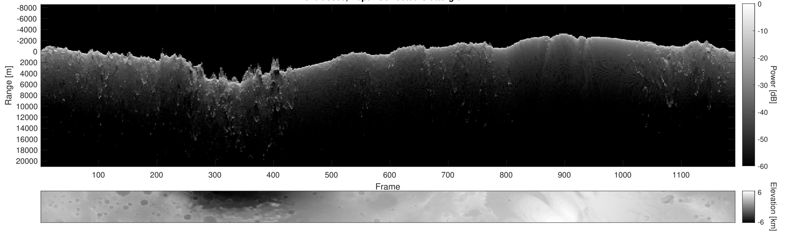
Orbit 8896, Depth-Corrected Cluttergram
