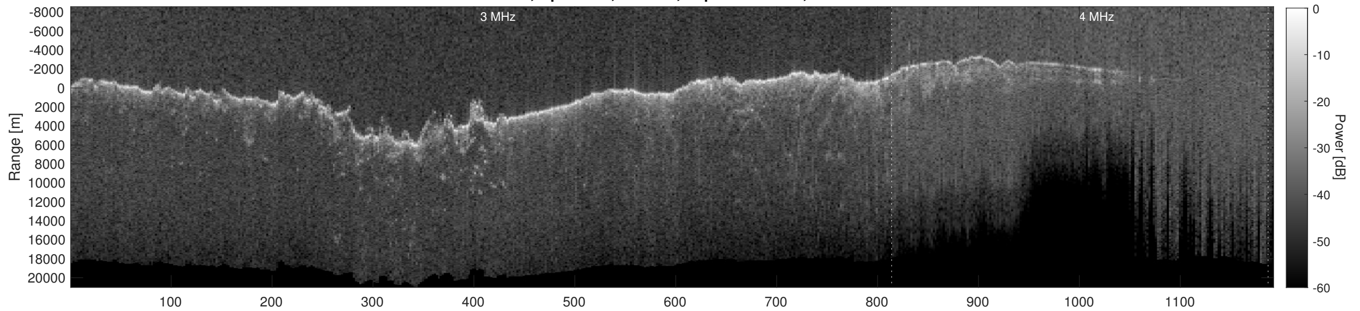
Orbit 8896, Depth-Corrected Cluttergram
