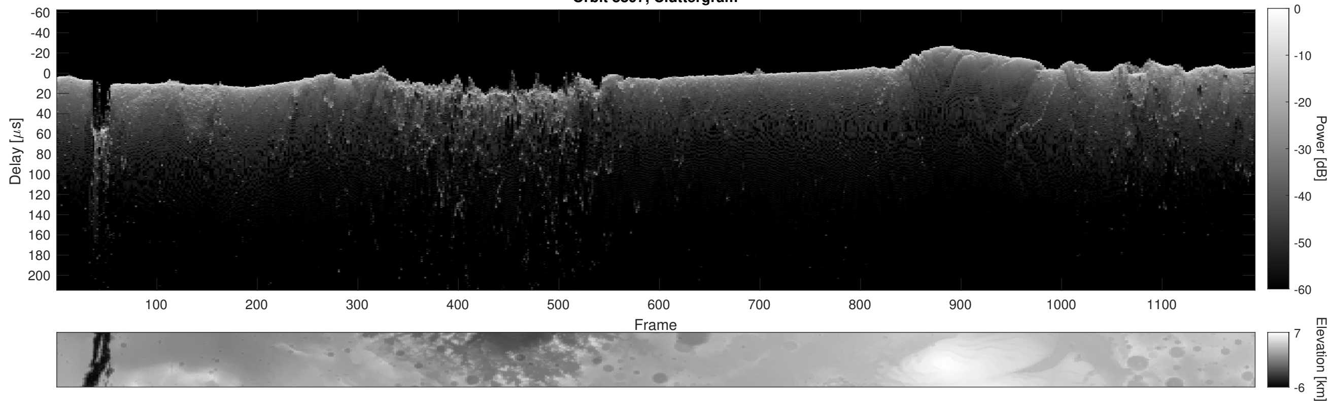
Orbit 8897, Cluttergram
