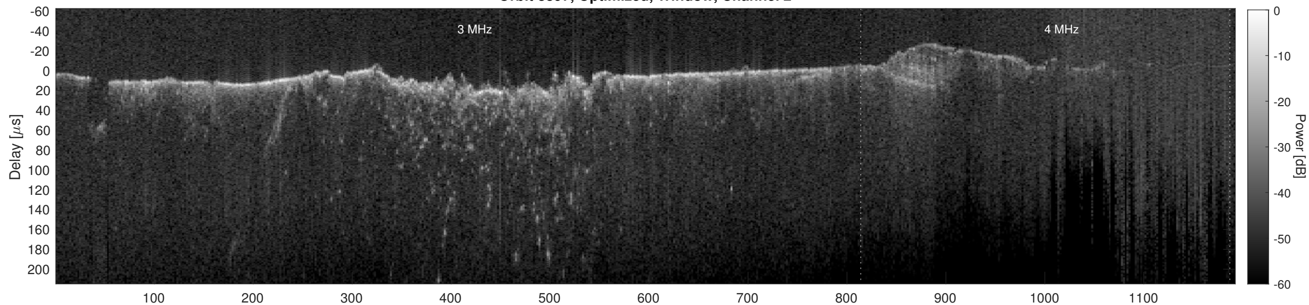
Orbit 8897, Cluttergram
