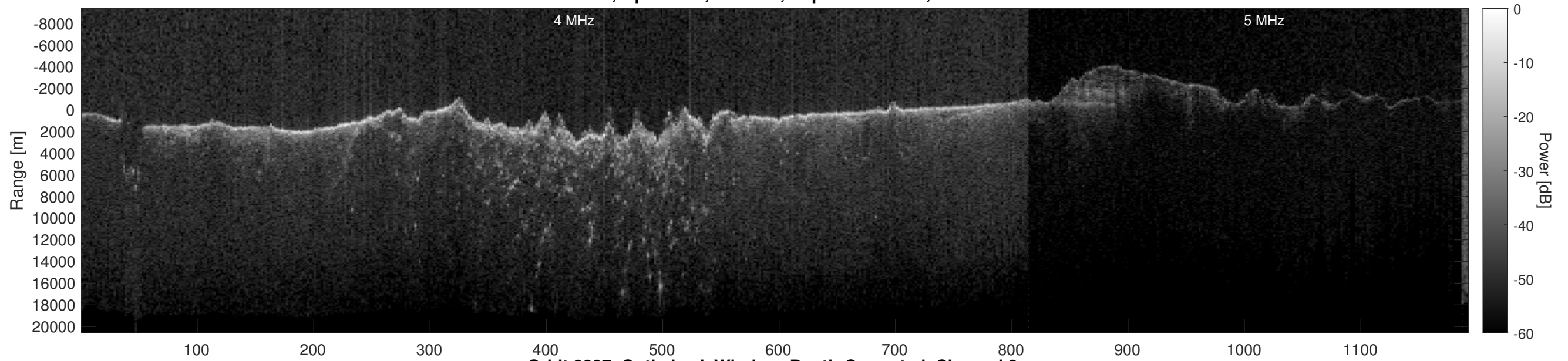
Orbit 8897, Optimized, Window, Depth-Corrected, Channel 2
