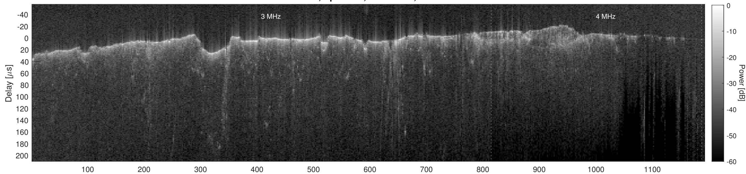
Orbit 8898, Cluttergram
