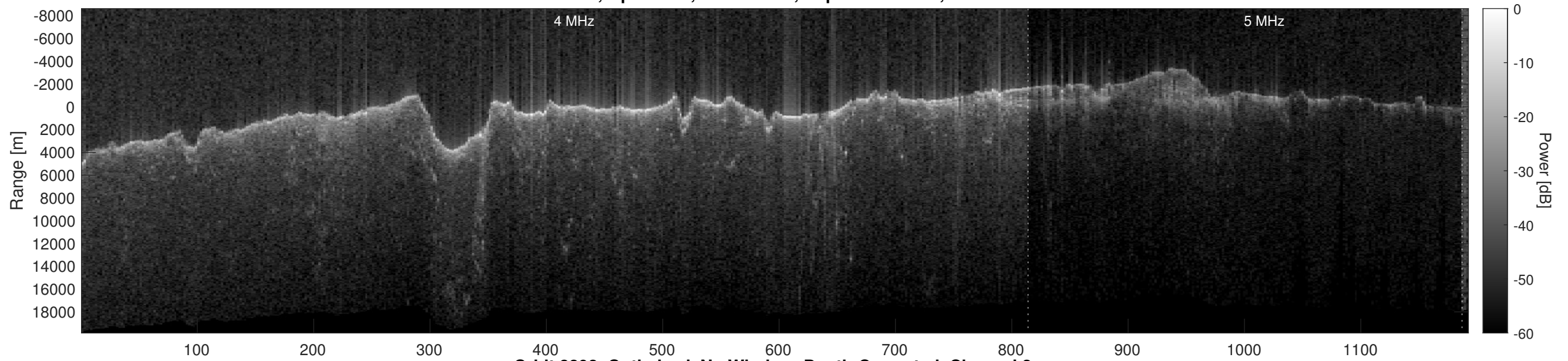
Orbit 8898, Optimized, No Window, Depth-Corrected, Channel 2
