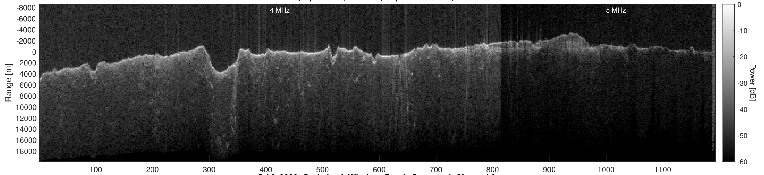
Orbit 8898, Optimized, Window, Depth-Corrected, Channel 2
