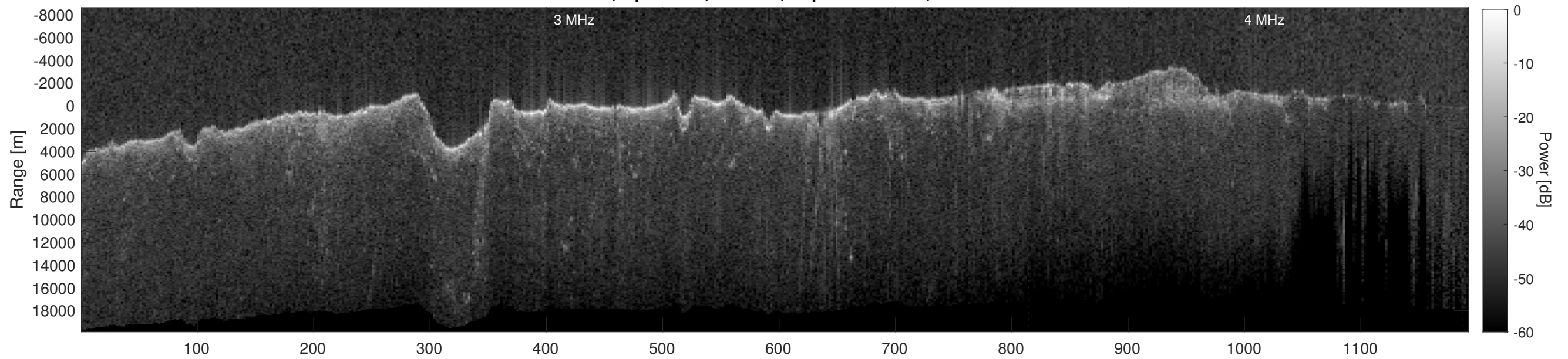
Orbit 8898, Depth-Corrected Cluttergram
