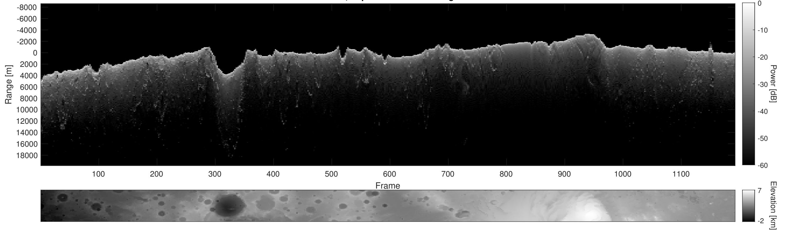
Orbit 8898, Depth-Corrected Cluttergram
