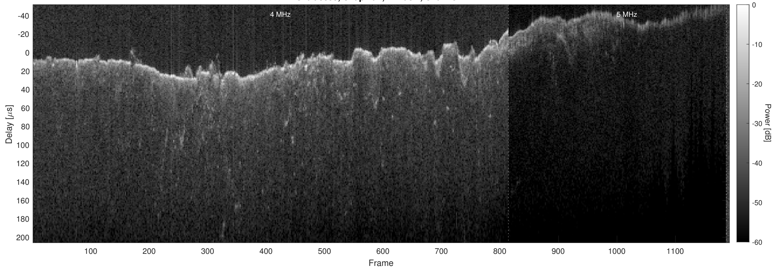
Orbit 8899, Chapman, Window, Channel 2
