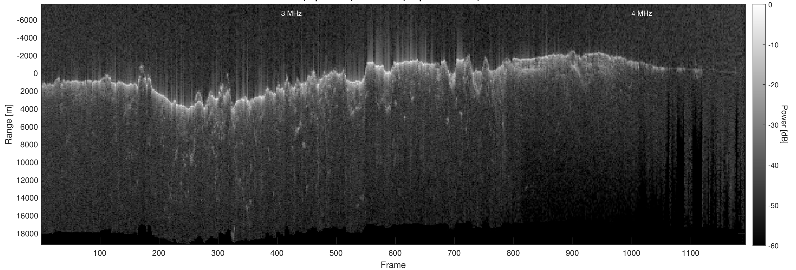
Orbit 8899, Optimized, No Window, Depth-Corrected, Channel 2
