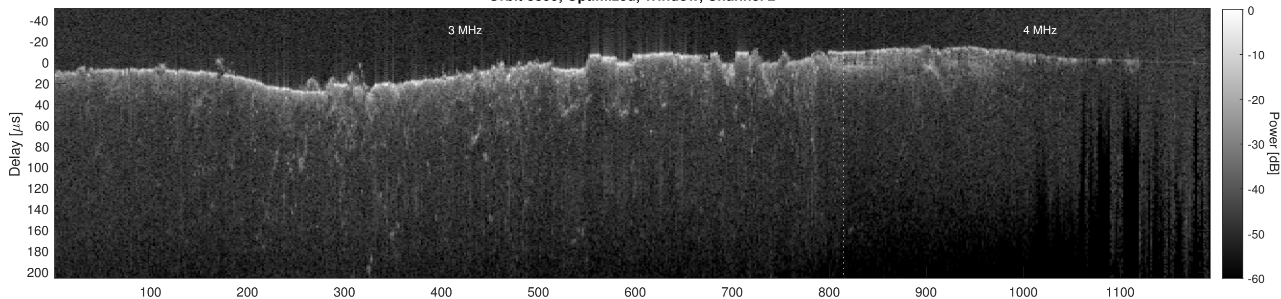
Orbit 8899, Cluttergram
