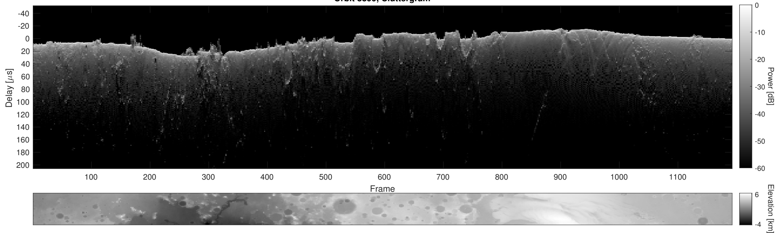
Orbit 8899, Cluttergram
