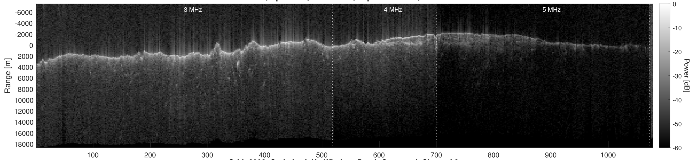
Orbit 8902, Optimized, No Window, Depth-Corrected, Channel 2
