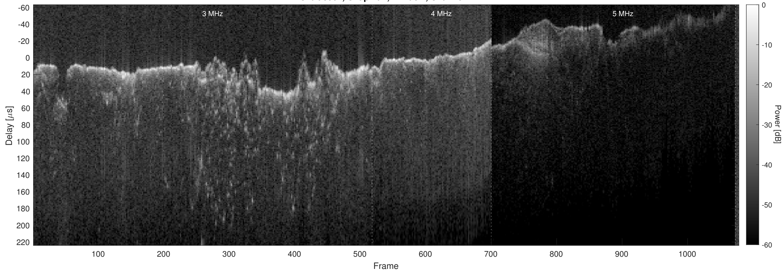
Orbit 8904, Chapman, Window, Channel 2
