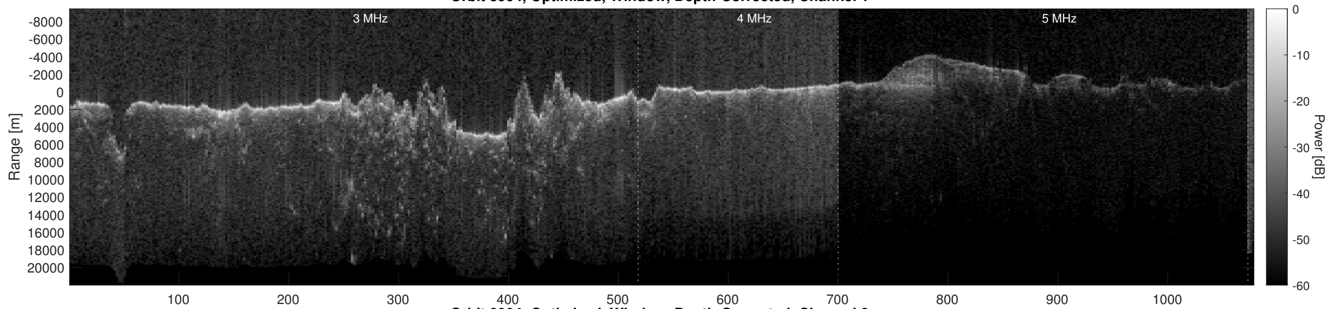
Orbit 8904, Optimized, Window, Depth-Corrected, Channel 2
