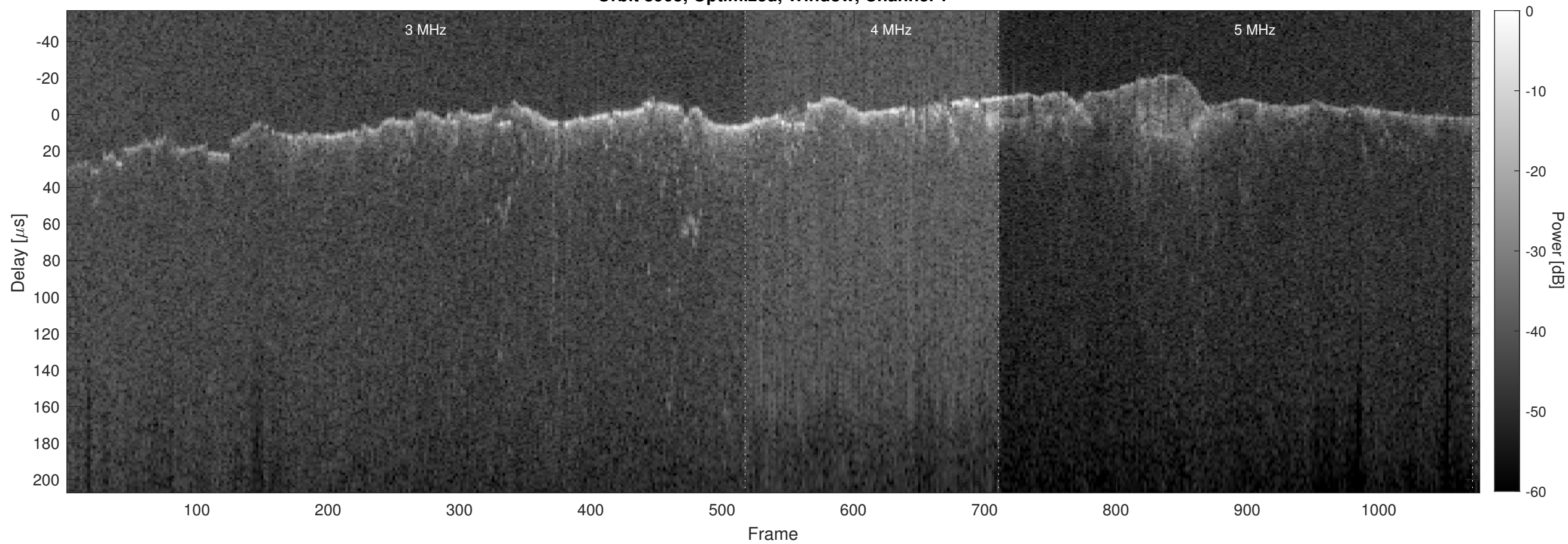
Orbit 8905, Optimized, Window, Channel 2
