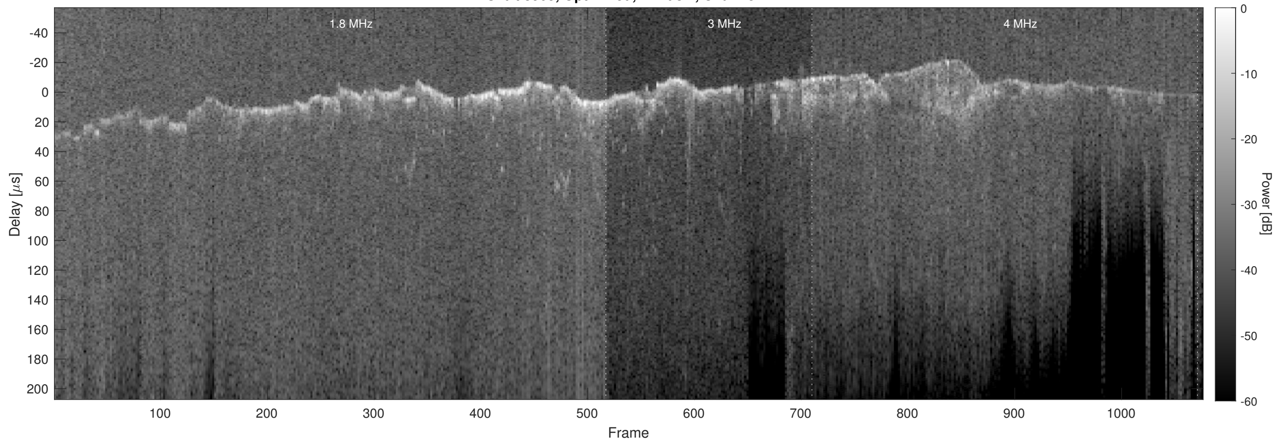
Orbit 8905, Optimized, Window, Channel 2
