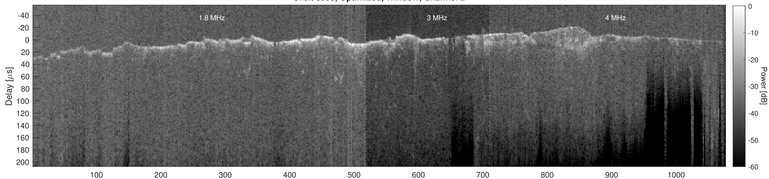
Orbit 8905, Cluttergram
