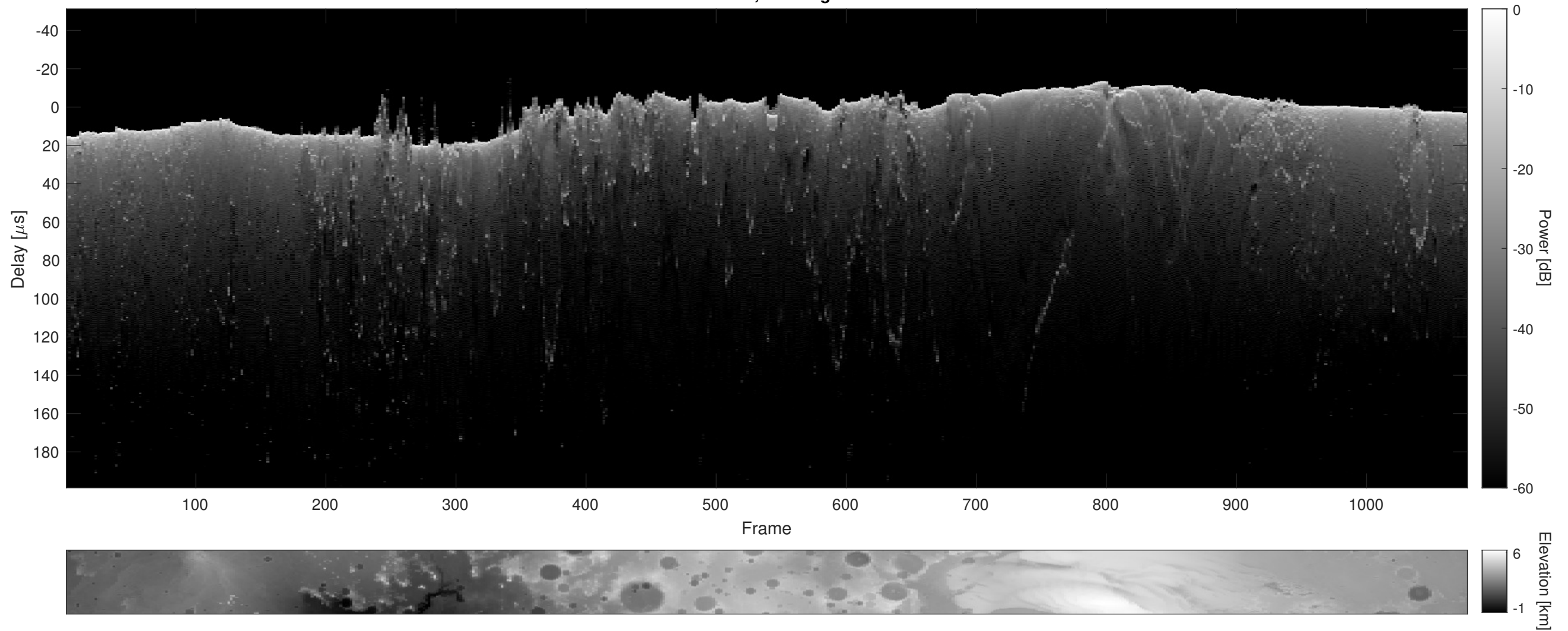
Orbit 8906, Cluttergram
