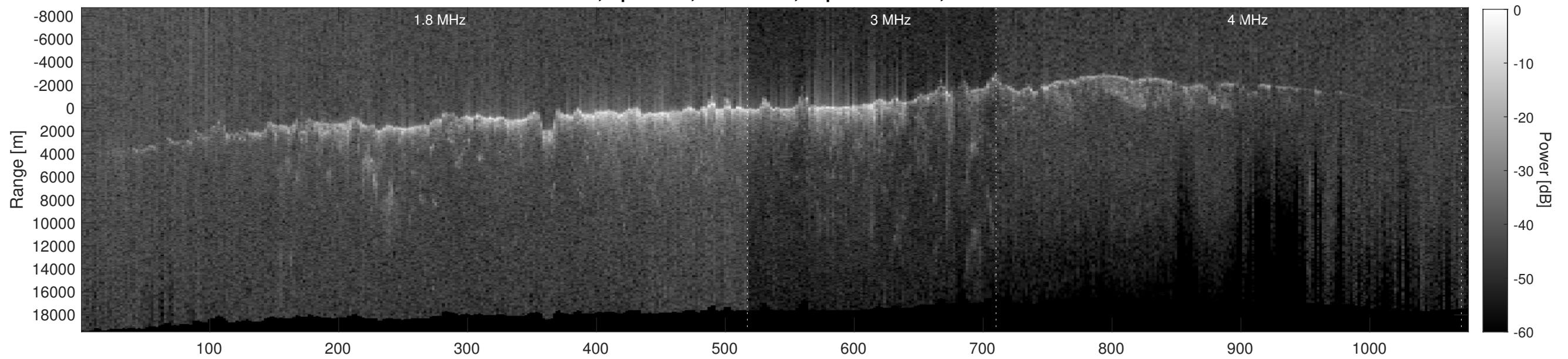
Orbit 8907, Depth-Corrected Cluttergram
