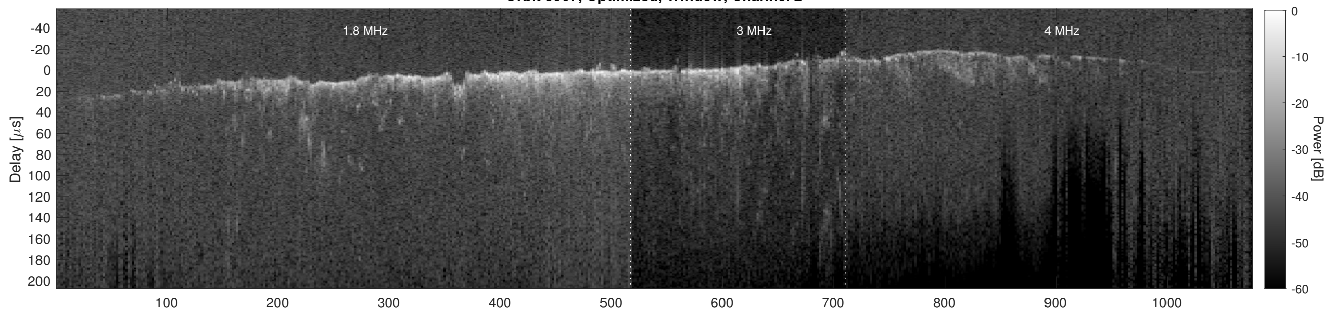
Orbit 8907, Cluttergram
