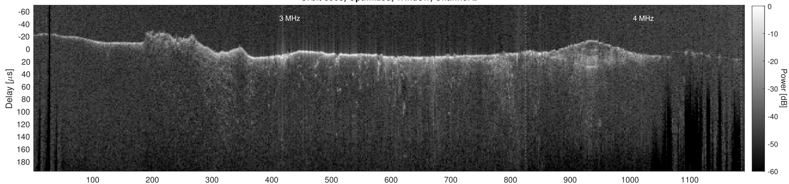
Orbit 8908, Cluttergram
