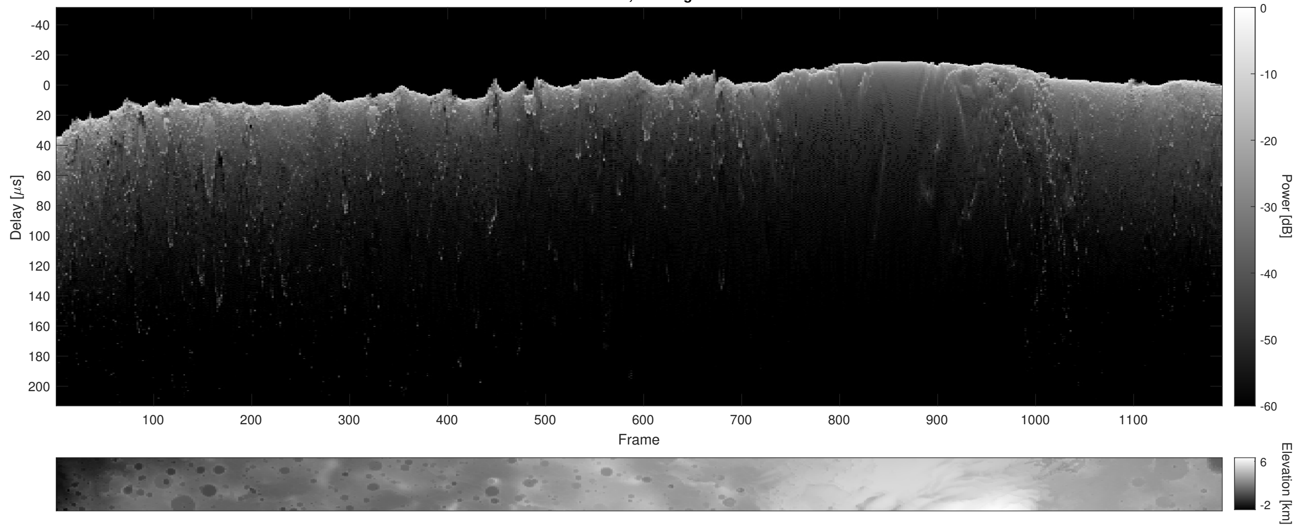
Orbit 8909, Cluttergram
