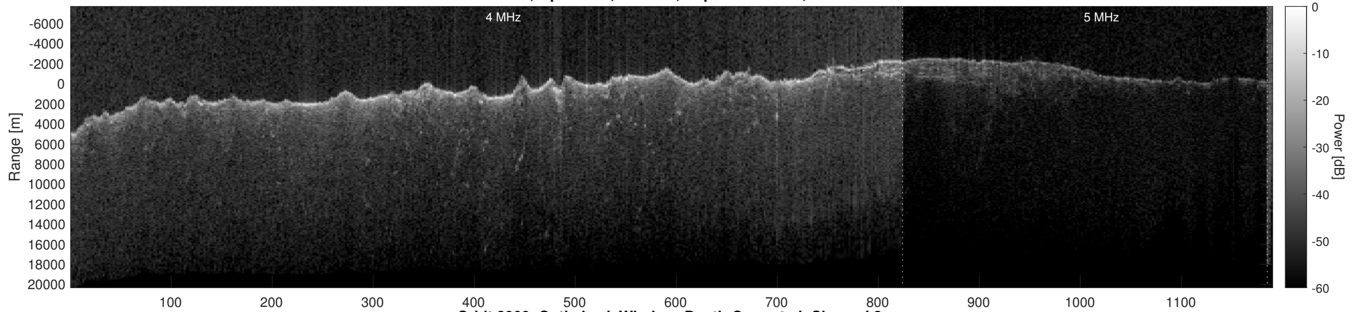
Orbit 8909, Optimized, Window, Depth-Corrected, Channel 2
