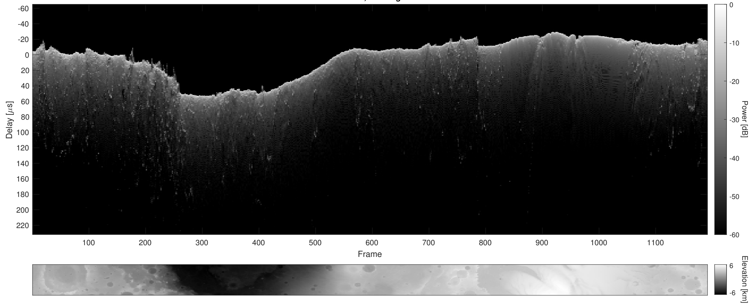
Orbit 8910, Cluttergram
