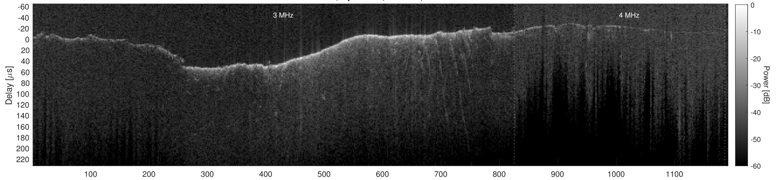
Orbit 8910, Cluttergram
