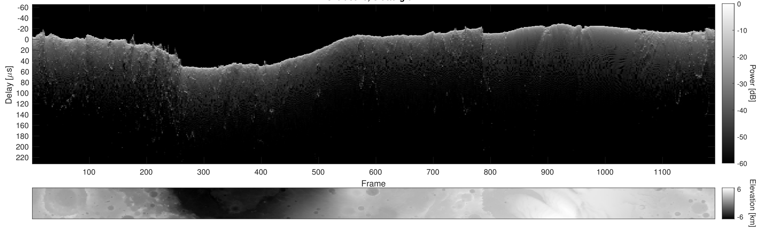
Orbit 8910, Cluttergram
