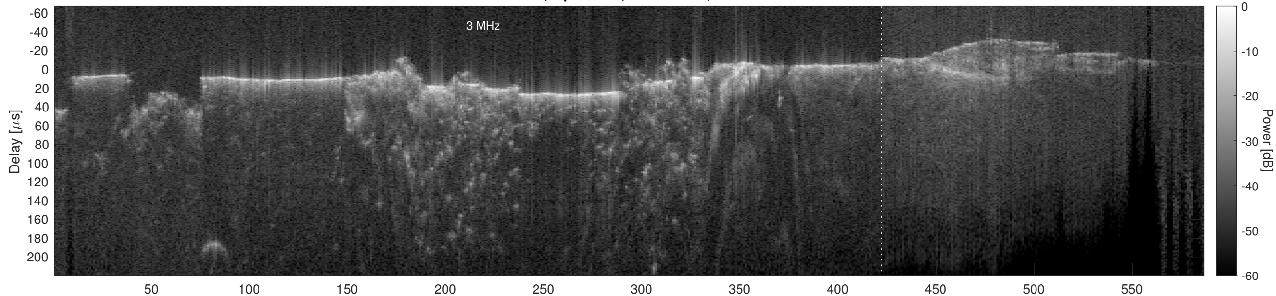
Orbit 8911, Optimized, No Window, Channel 2
