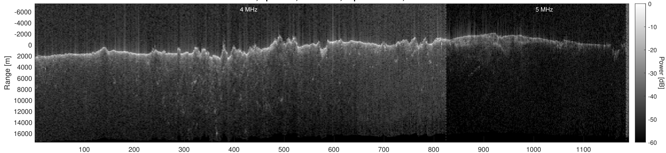
Orbit 8913, Optimized, No Window, Depth-Corrected, Channel 2
