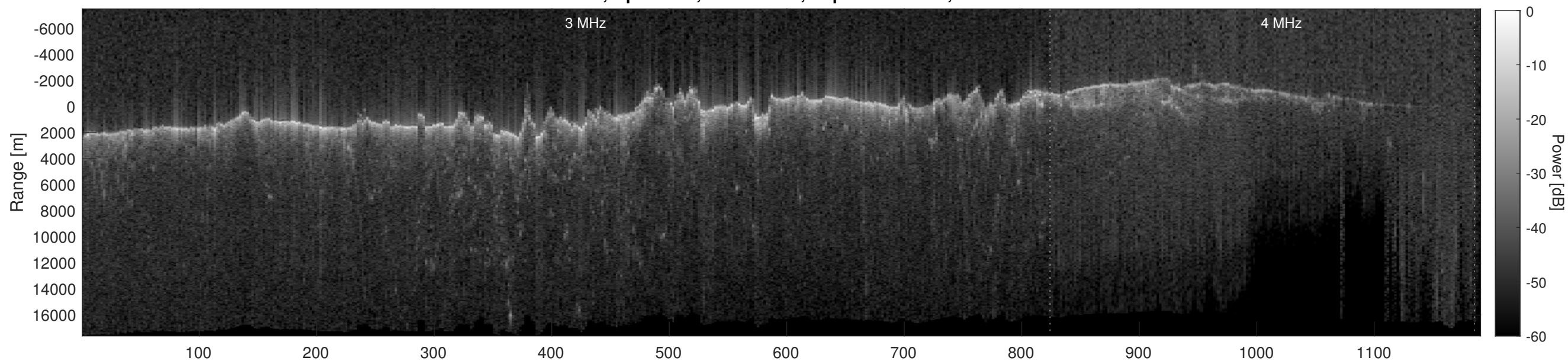
Orbit 8913, Depth-Corrected Cluttergram
