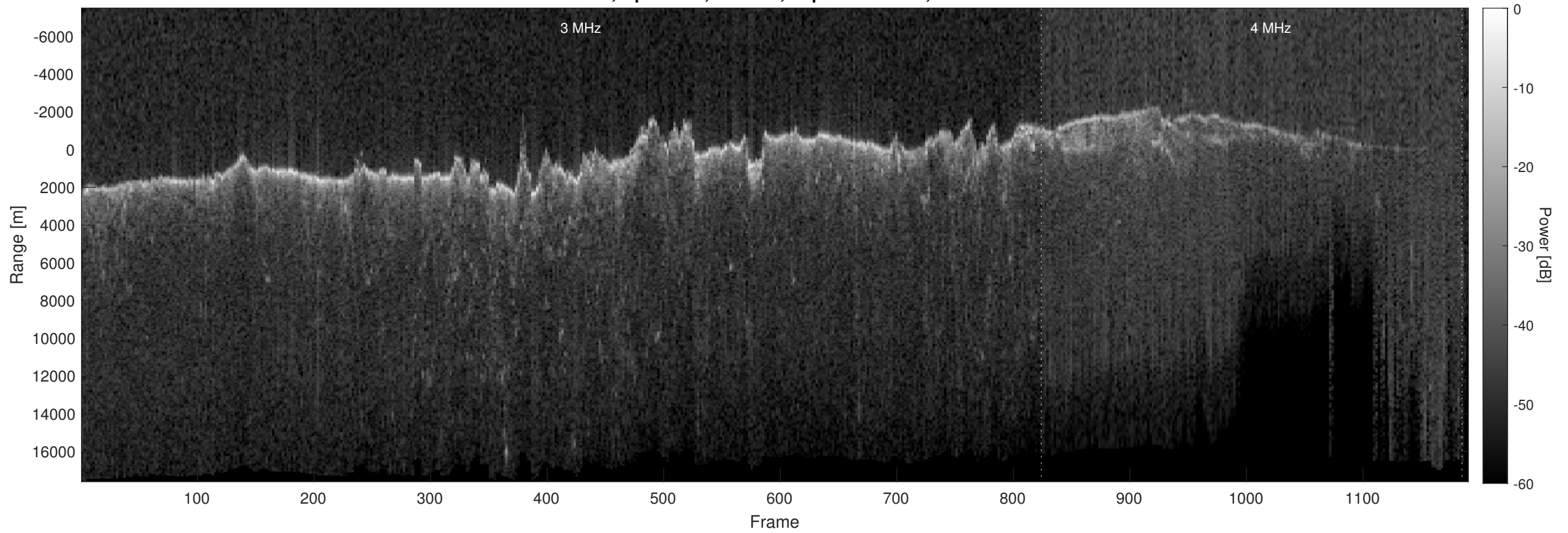
Orbit 8913, Optimized, Window, Depth-Corrected, Channel 2
