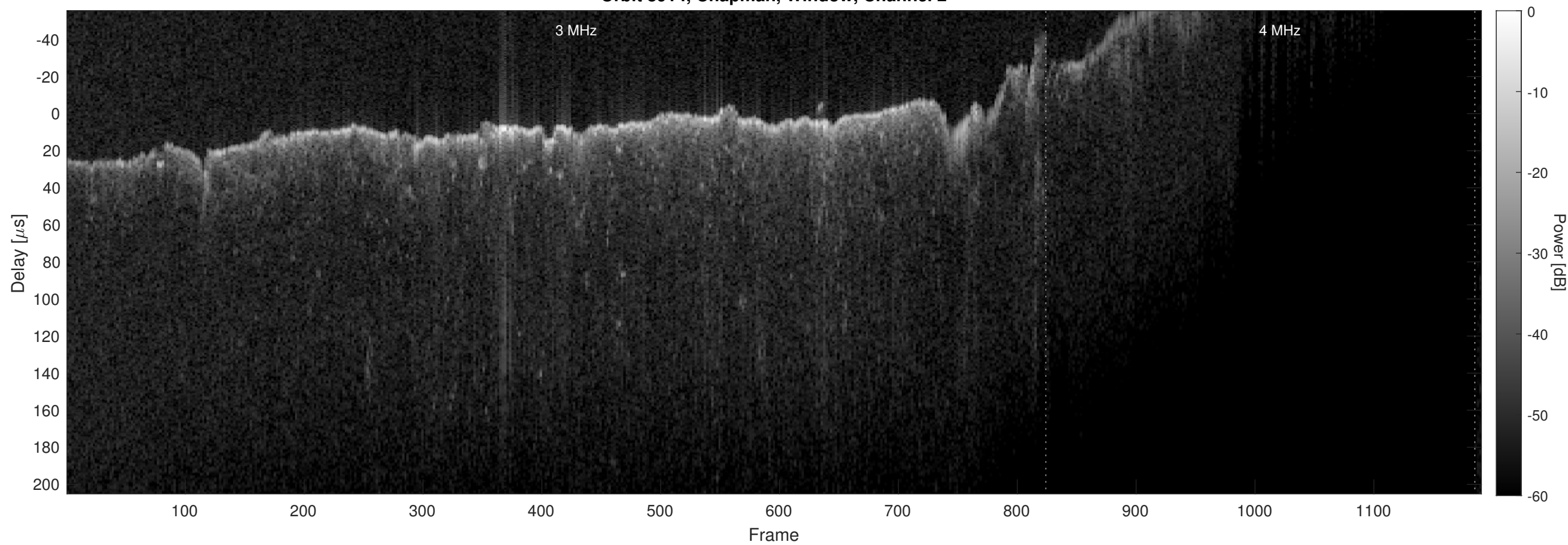
Orbit 8914, Chapman, Window, Channel 2
