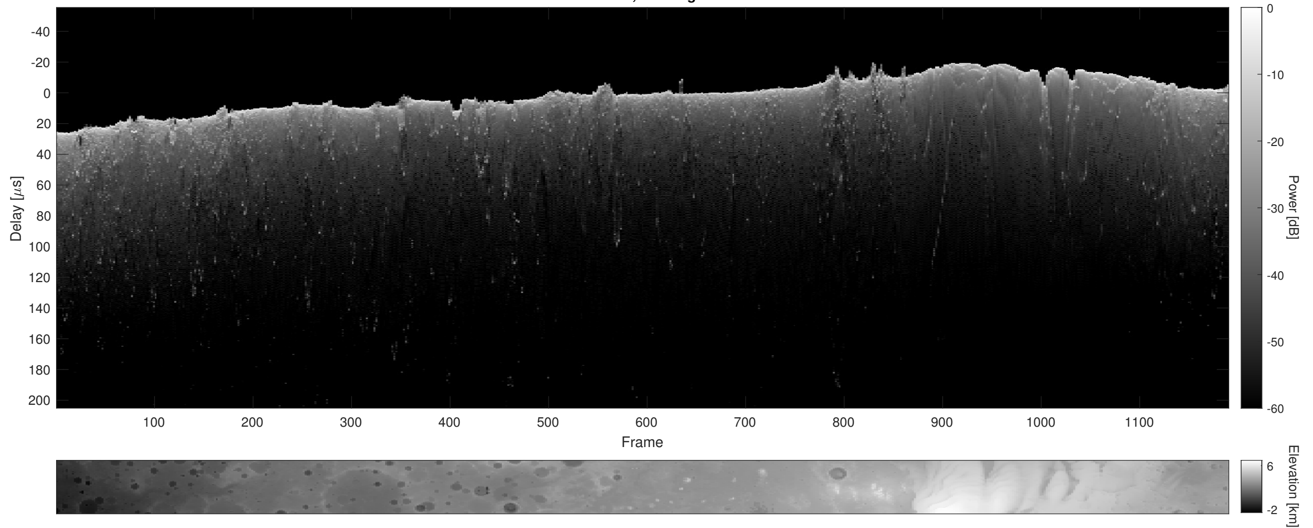
Orbit 8914, Cluttergram
