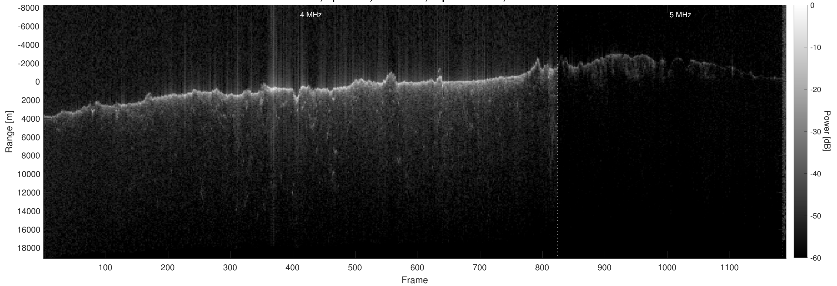
Orbit 8914, Optimized, No Window, Depth-Corrected, Channel 2
