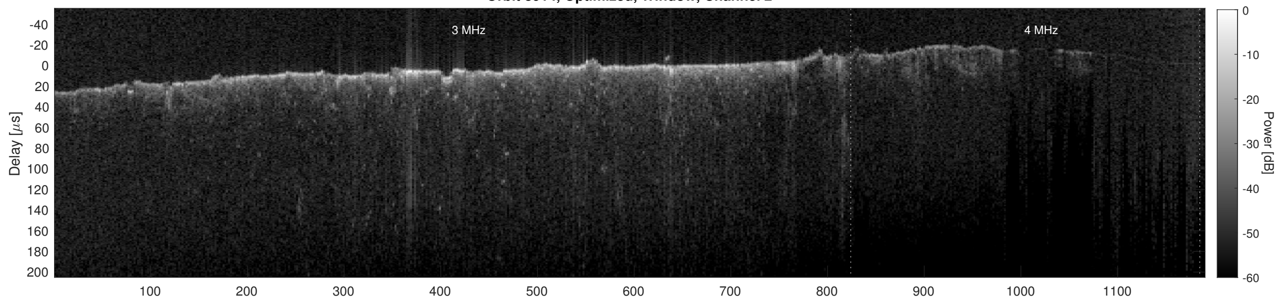
Orbit 8914, Cluttergram
