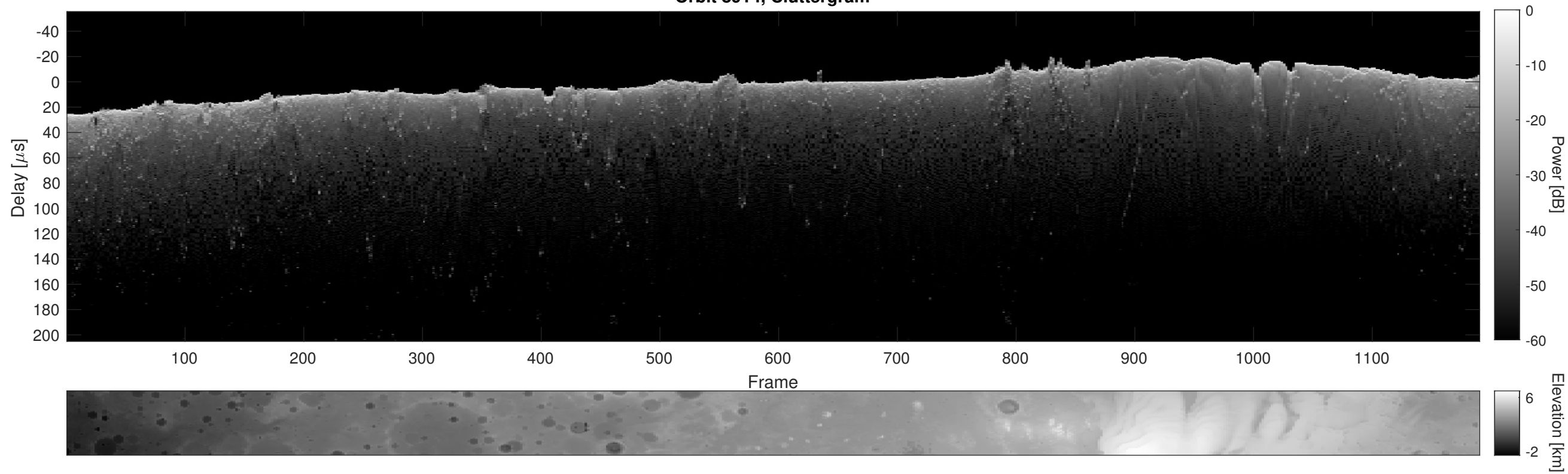
Orbit 8914, Cluttergram
