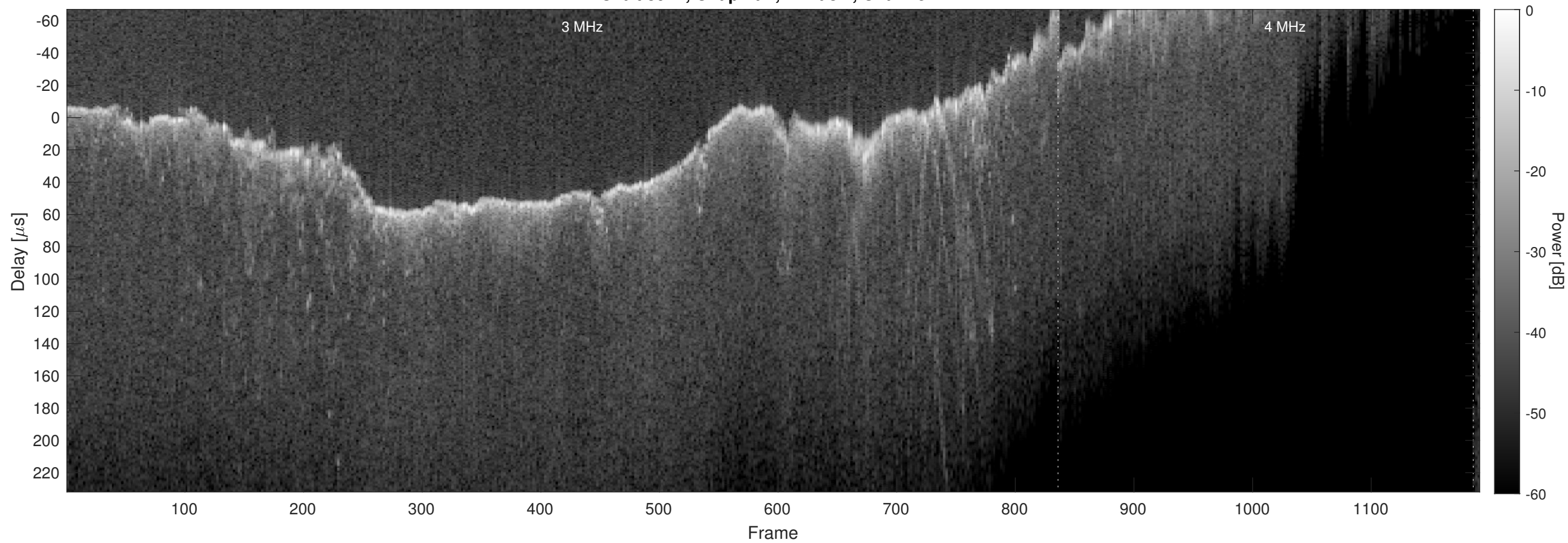
Orbit 8917, Chapman, Window, Channel 2
