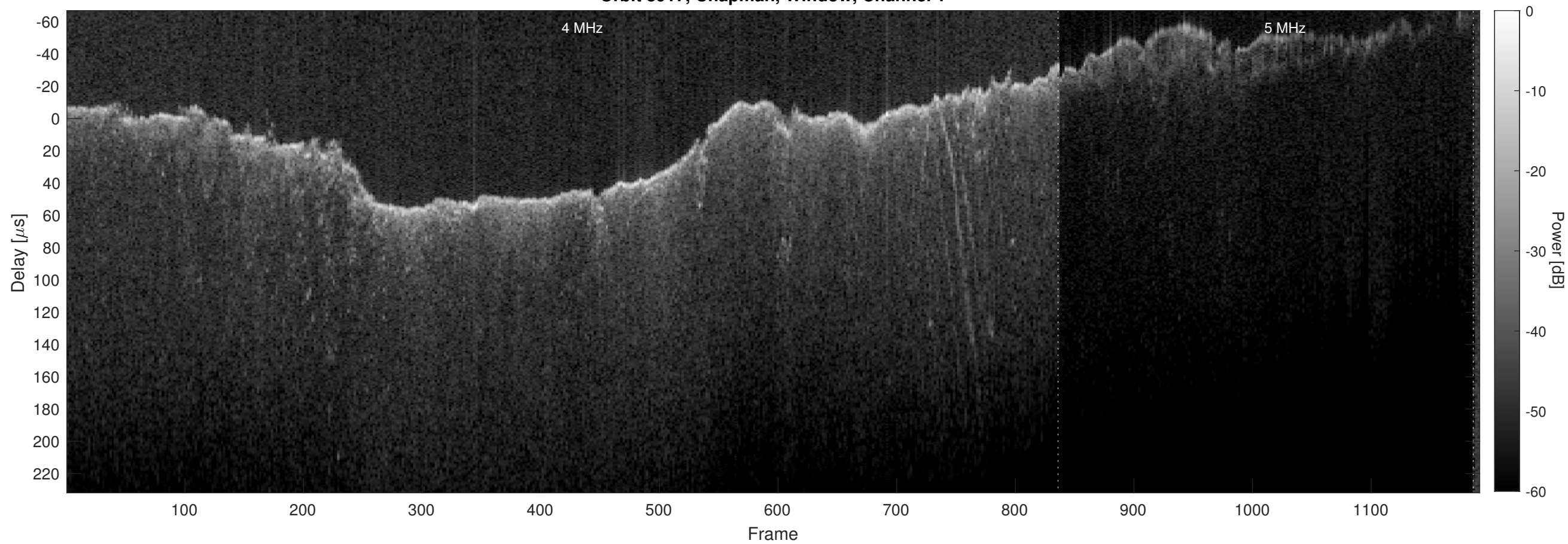
Orbit 8917, Chapman, Window, Channel 2
